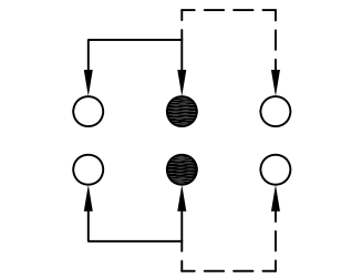
SCHEMATIC (NON-SHORTING)
